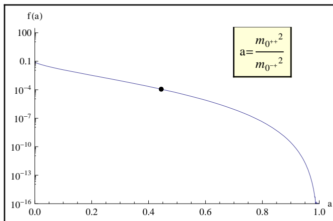
Figure 3. Kinematic suppression factor f(a) . Point corresponds to a value of a taken for v -glueball masses from the Morningstar and Peardon spectrum [11].
