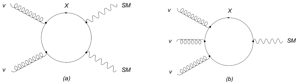
Figure 2. Diagrams contributing to the effective action
