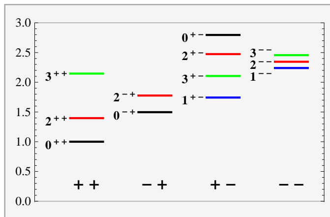
Figure 1. Spectrum of stable glueballs in pure glue SU(3) theory [11].
